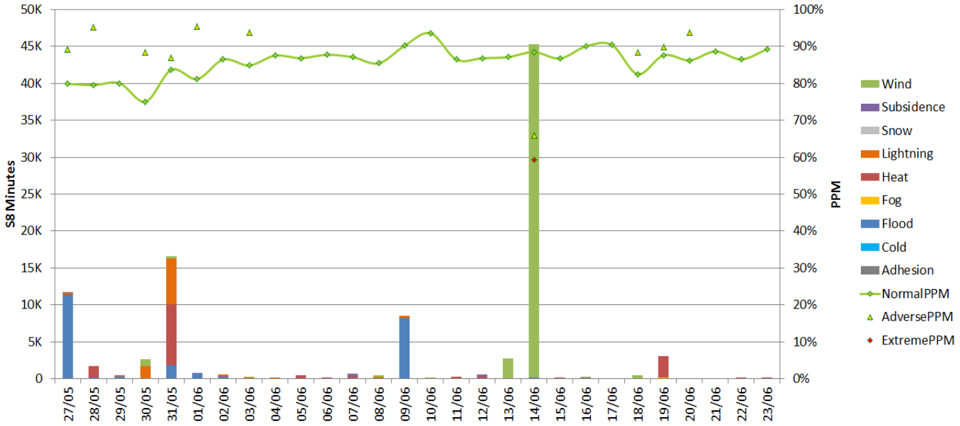
Figure 1 Weather related PPM and delay minutes for P3 2018
