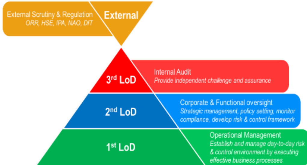
Figure 19 Assurance model
