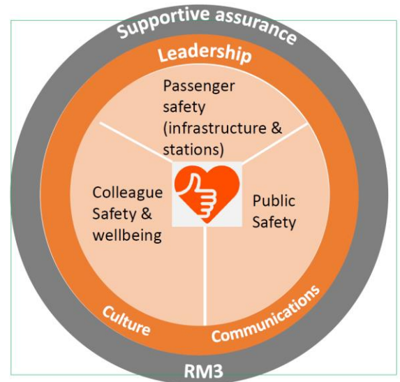
Figure 4 Safety Framework
