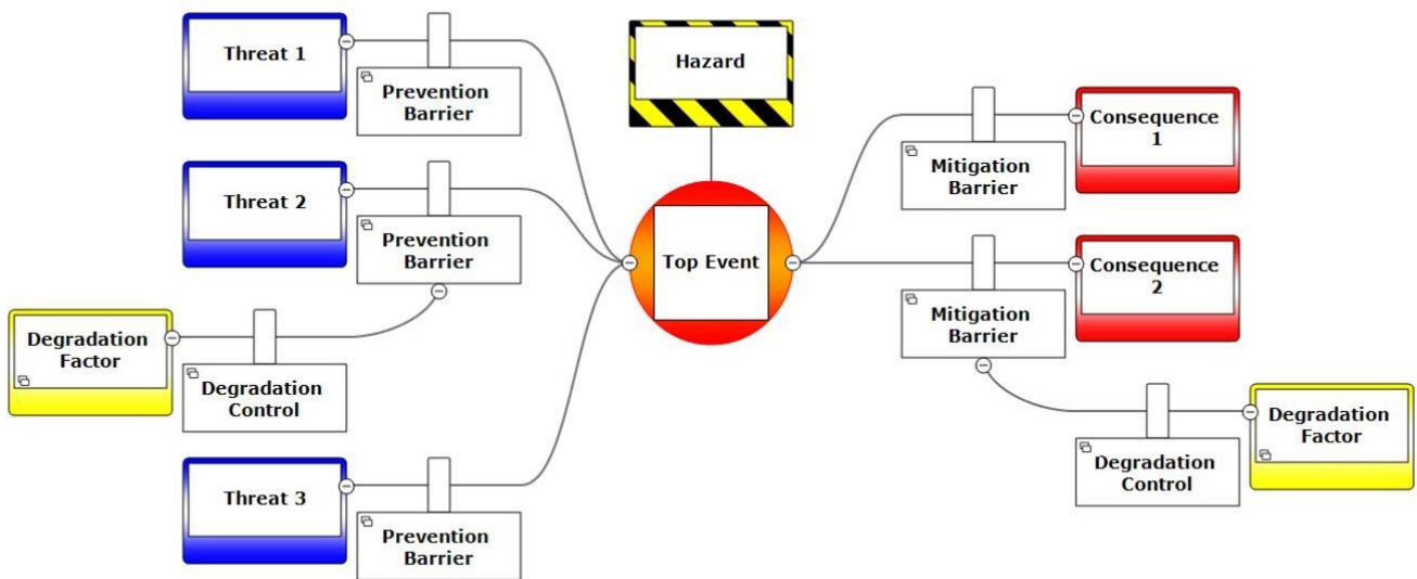
Figure 13 Bow-tie risk assessment (RSSB 2023)
